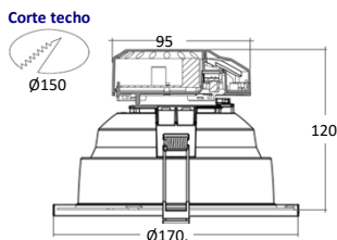
ASTROLUX-150-20W-2200lm/840
