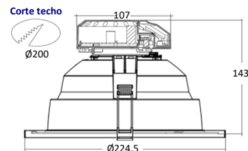
ASTROLUX-200-20W-2200lm/840 ASTROLUX-200-30W-3200lm/840
