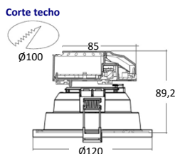
ASTROLUX-100-10W-1100lm/840
