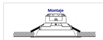
ASTROLUX-200-20W-2200lm/840 ASTROLUX-200-30W-3200lm/840
